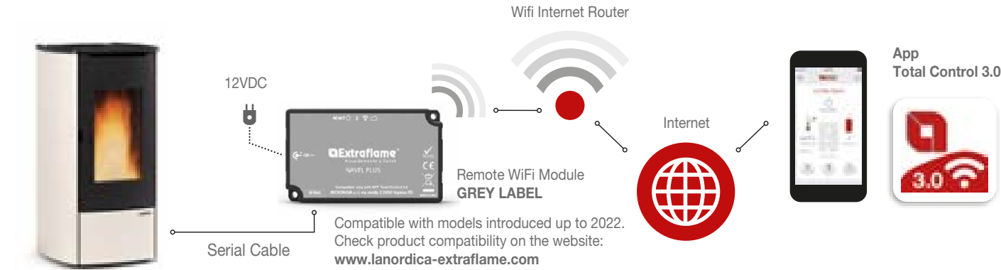
Remote WiFi Module diagram "GREY LABEL" (C)
